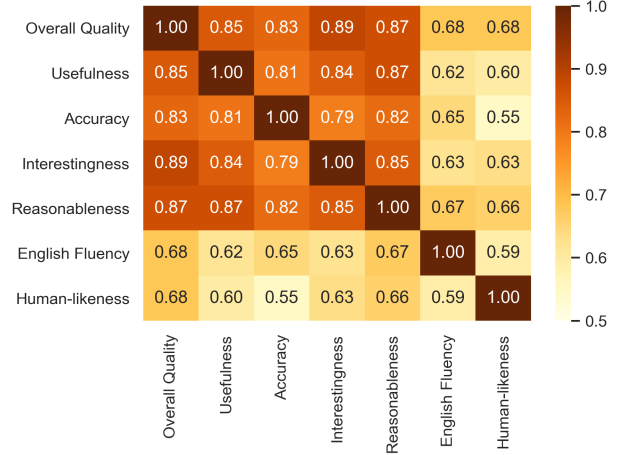
Figure 3: Pearson’s correlation of response quality.
